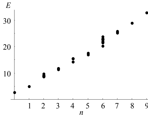
Figure 2. Dependence of energies of motifs on number of quanta in a given mode for fuga BWV 847. Graphs show coincidence of energies calculated by equations (2) and (4).
