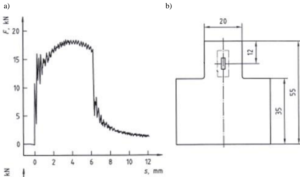
Figure 2. a) Force-displacement curve, b) sketch of the instrumented knife [6].
